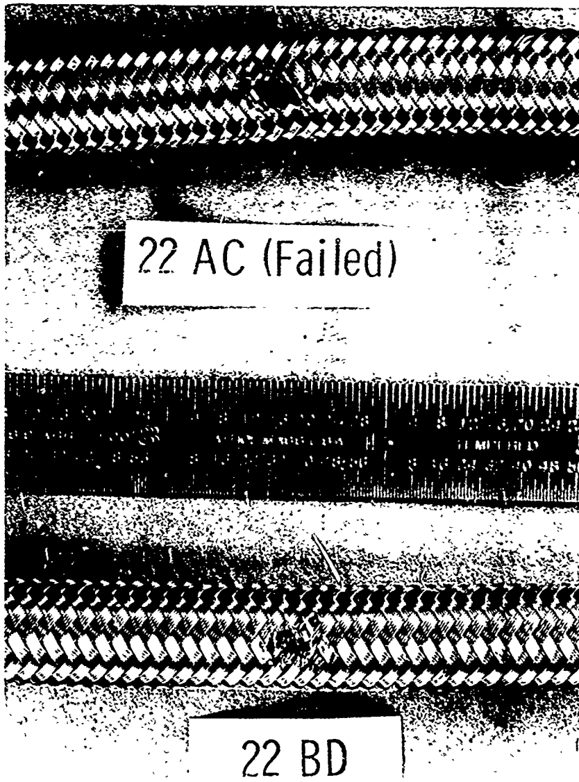
Figure 10. Test Specimens 22AC and 22BD.
